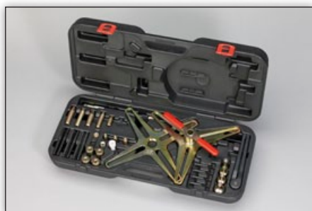
Fig. 2: SAC-gereedschapskoffer 400 0237 10
